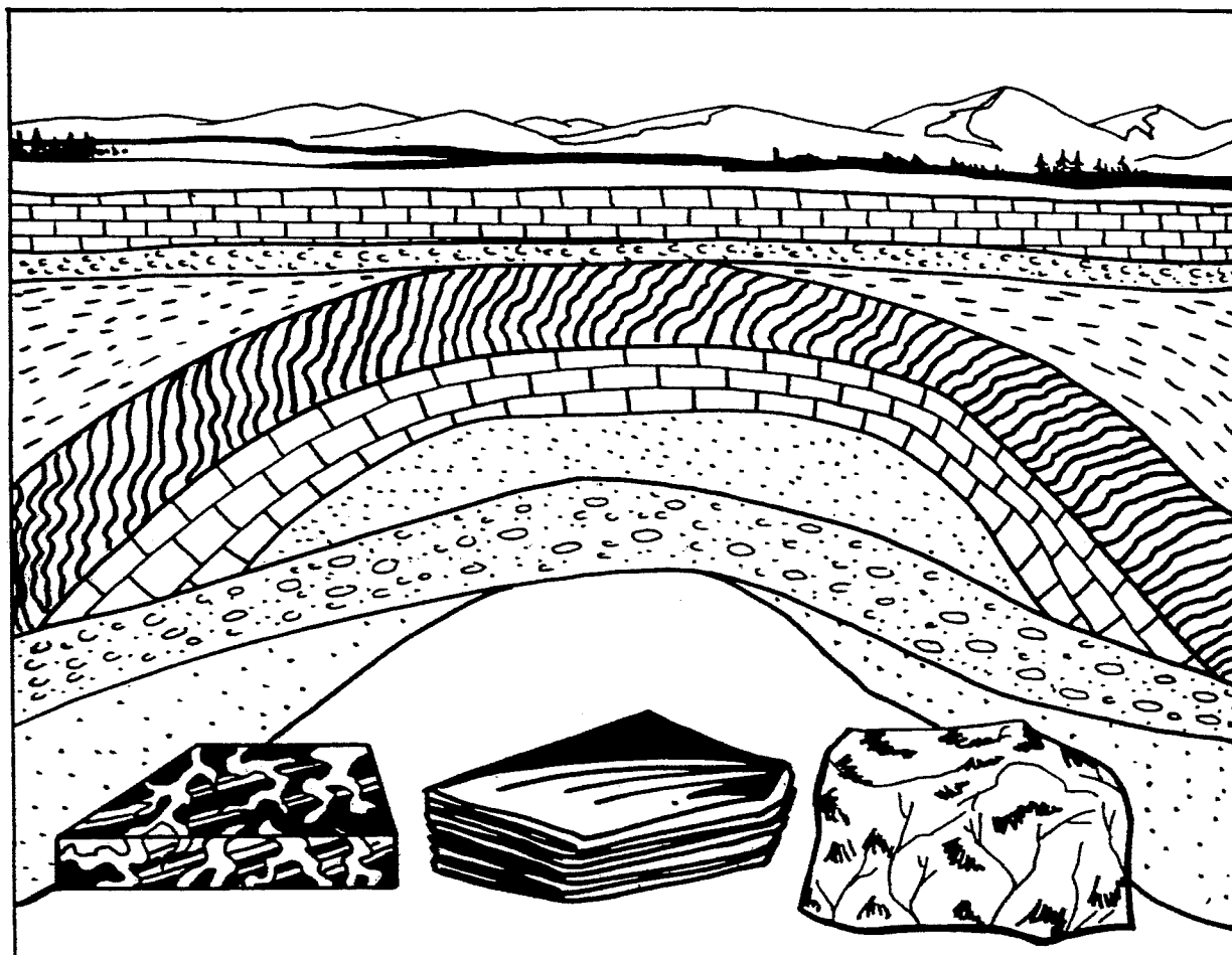
Metamorphic rocks such as marble, slate, and quartzite are formed when heat, pressure, and chemical action change igneous and sedimentary rocks.
